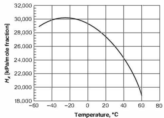
FIGURE F.2.1.2(b) HFC-125: Henry's Law Constant, H_x , for Nitrogen Solubility, SI Units.
